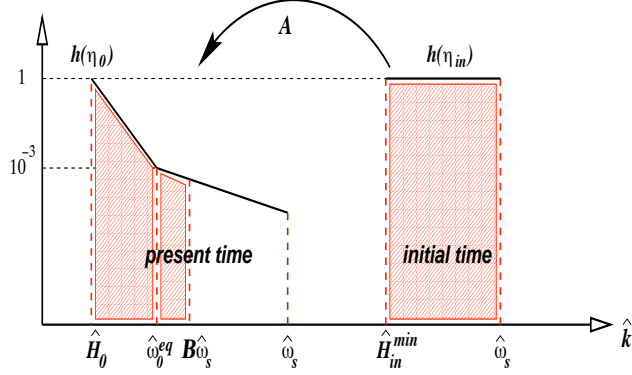
FIG. 2. We show schematically how the “transfer function” between initial and present time acts both on the amplitude, Eq. (2.25), and the frequency, Eq. (2.26), of tensor fluctuations. We have assumed for simplicity that h(\eta_{\text{in}}) = 1 and \bar{g}_{\text{in}} = 1 . In the minimal PBB scenario the initial string frequency \hat{\omega}_s = \lambda_s^{-1} corresponds today to B\hat{\omega}_s = 1 Hz. The present Hubble frequency \hat{H}_0 = B\hat{H}_{\text{in}}^{\text{min}} \sim 10^{-18} Hz originates from the initial frequency \hat{H}_{\text{in}}^{\text{min}} \sim 10^{24} Hz, which corresponds to 1 Fermi. Note that, whereas the colored regions refer to initial classical fluctuations, the white one on the left part of the figure concerns wavelengths that would correspond to initial length scales formally smaller than the string scale, i.e. to quantum fluctuations. For them the classical transfer function does not apply.
