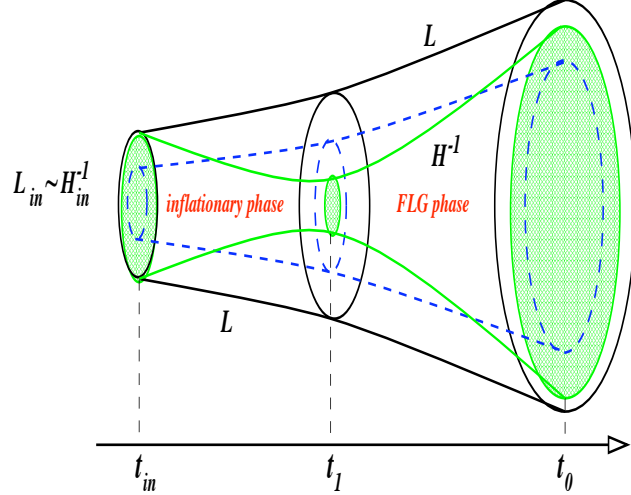
FIG. 1. Schematic representation, in the string frame and for the nonminimal version of the PBB scenario, of the evolution of: the Hubble horizon H^{-1} , an intermediate physical wavelength (dashed line) and the comoving size L (continuous line) corresponding to the initial patch H^{-1} .
