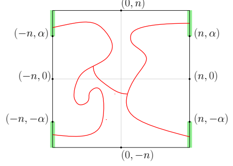
Figure 2: A diagrammatic representation of the event \mathcal{X}_n(\alpha)
