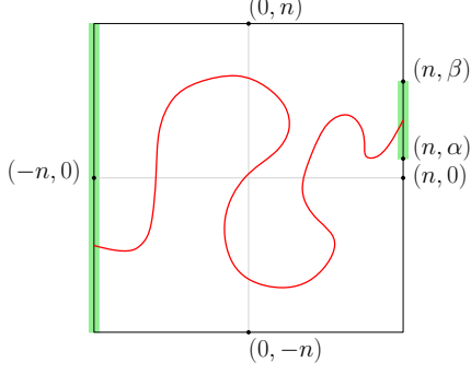
Figure 1: A diagrammatic representation of the event \mathcal{H}_n(\alpha, \beta)
