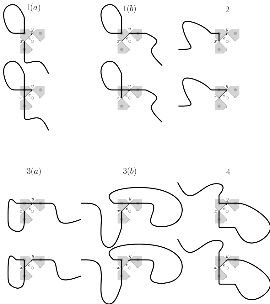
Figure 9.1: The different possible cases in the proof of Theorem 9.5: \omega is depicted at the top, and \omega' at the bottom of each case.
