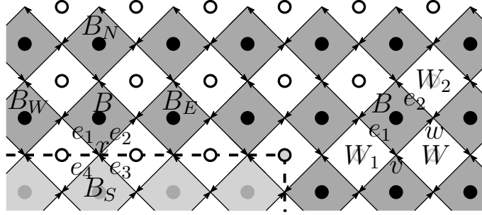
Figure 8.2: Extend \Omega_\delta^\circ by adding one extra layers of medial faces, and extend the functions H_\delta^\bullet on these new medial faces. On the right, the indexation of faces and edges for the proof of Lemma 8.35.
