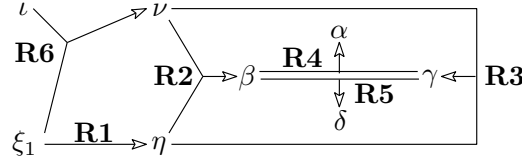
Figure 13.2: How exponents would follow from \xi_1 and \iota .
