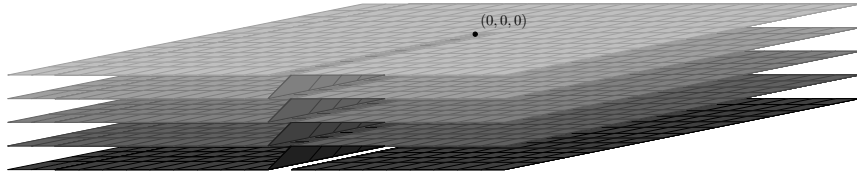
Figure 6.4: The graph \mathbb{U} .
