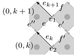
Figure 11.1: The labeling of medial-edges around e_k and e_{k+1} used in Step 1.
