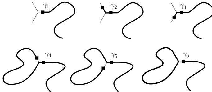
Figure 12.2: Following the same proof as for self-avoiding walks, one may associate configurations \gamma_1, \gamma_2 and \gamma_3 (resp. \gamma_4, \gamma_5 and \gamma_6 ) together to show that the sum of contributions vanishes in Proposition 12.12 (note the additional configuration with one self-avoiding walk visiting one mid-edge around the vertex and a loop facing it). We leave the proof as an exercise.
