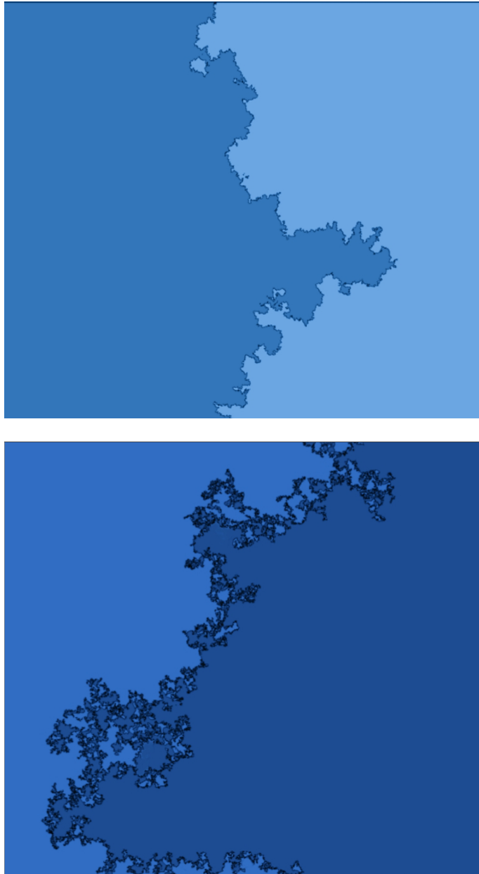
Figure 1.4: Two examples of Schramm-Loewner Evolutions (SLE(8/3) and SLE(6)). The behavior is very different: the first one is almost surely a simple curve (i.e. non intersecting) while the second one has self-touching points. The Hausdorff dimensions are also different. (© V. Beffara).
