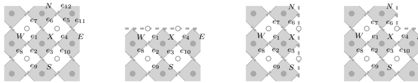
Figure 11.2: Indexation of the edges around vertices in the different cases.
