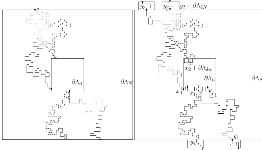
Figure 10.5: On the left, the four-arm event A_{1010}(n, N) . On the right, the event A_{1010}^{sep}(n, N) with well-separated arms. Note that these arms are not at macroscopic distance of each other inside the domain, but only at their end-points.
