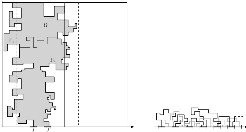
Figure 5.6: The construction in Case 1 with the two paths \Gamma_1 and \Gamma_2 and the domain \Omega between the two paths. On the right, a combination of paths creating a long path from left to right.
