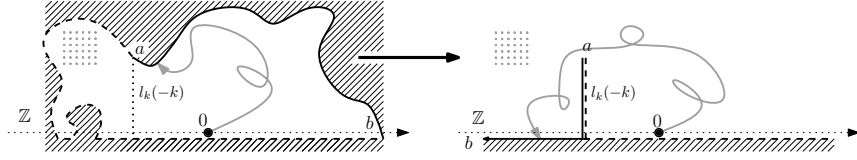
Figure 10.1: The two domains involved in the proof of Lemma 10.3.
