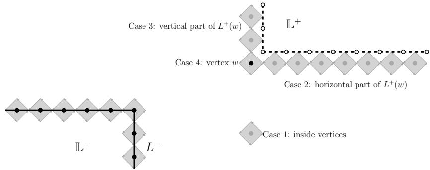
Figure 11.3: The set T(w) . The different cases listed in the definition of the Laplacian are also depicted.
