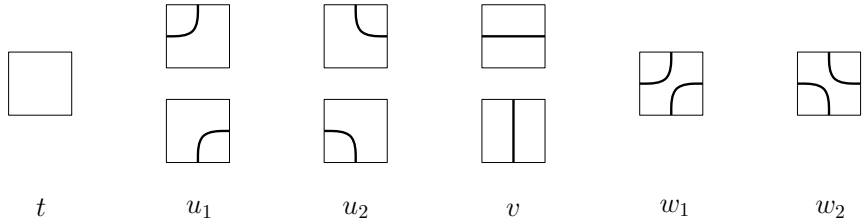
Figure 12.3: Different possible plaquets with their associated weights.
