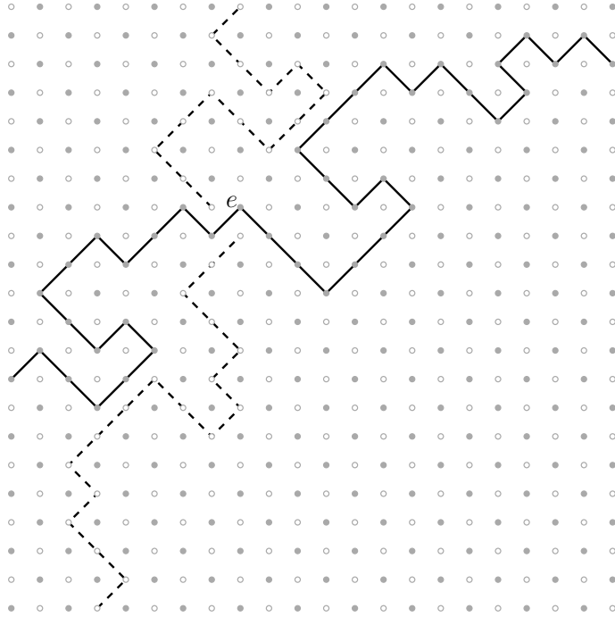
Figure 5.2: The square [0, n]^2 and its dual. The event \mathcal{C}_n([0, n]^2) is occurring. If the right edge e is turned to closed, then \mathcal{C}_v^*([0, n]^2) occurs.
