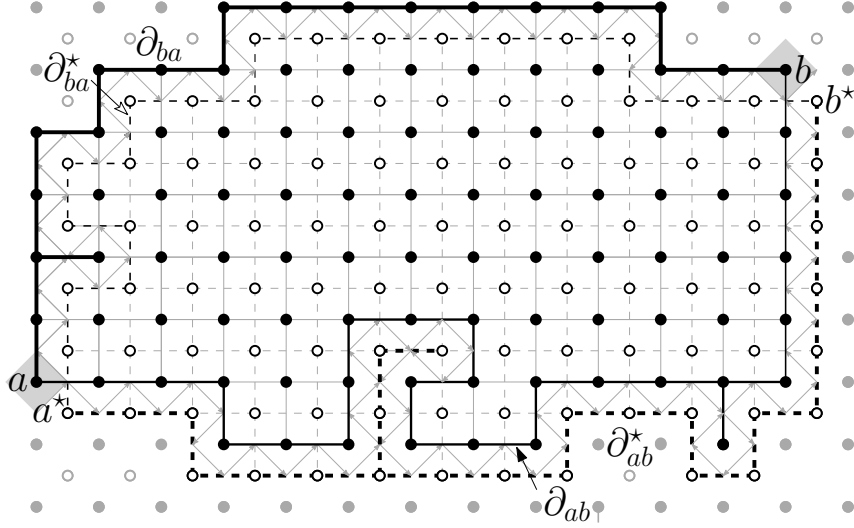
Figure 3.6: The primal and dual Dobrushin domains associated to a medial Dobrushin domain. Note the position of a , a^* , b and b^* .
