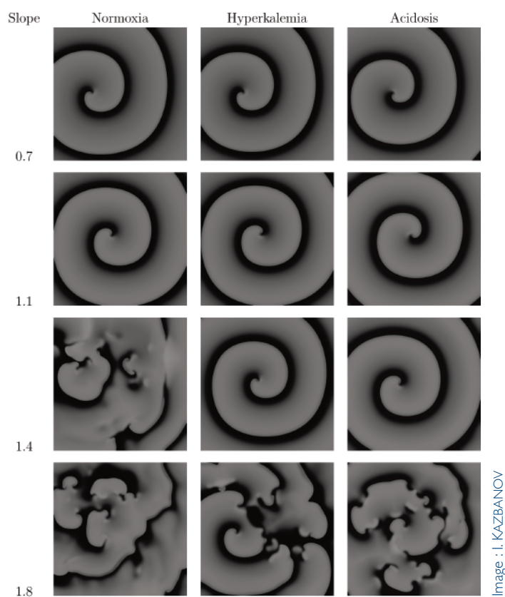
Effects of specific factors of ischemia on spiral wave reentry for different slopes of the cardiac restitution curves
