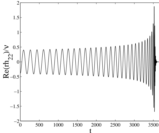
Figure 3: This figure illustrates a complete resummed EOB quadrupolar ( \ell = 2 , m = 2 ) waveform (28) (using a_5 = 20 , \bar{a}_{RR} = 30 and a suitably flexed v_{\text{pole}} ), with, about, 29 GW cycles of inspiral, \sim 1 GW cycle during plunge, and \sim 4 GW cycles of ring-down. Ref. [24] has shown that the inspiral part of the EOB waveform agreed with the Caltech-Cornell NR data [17] within \pm 0.001 GW cycles, while Ref. [25] has shown that the late-inspiral-plunge-ringdown part of the EOB waveform agrees with an Albert Einstein Institute NR waveform within \pm 0.005 GW cycles.
