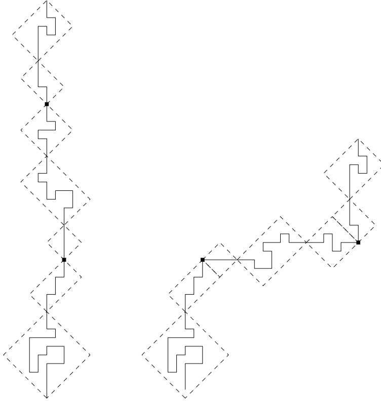
FIGURE 3. The stickbreak operation is depicted.
