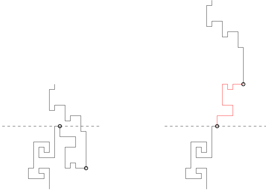
FIGURE 4. In the left-hand sketch, an element of \text{SAB}_n and one of its zigzags is illustrated. The zigzag's central section is shown in red and the points of zig and of zag are marked by circles. The unfolding of the walk indexed by this zigzag is depicted on the right.
