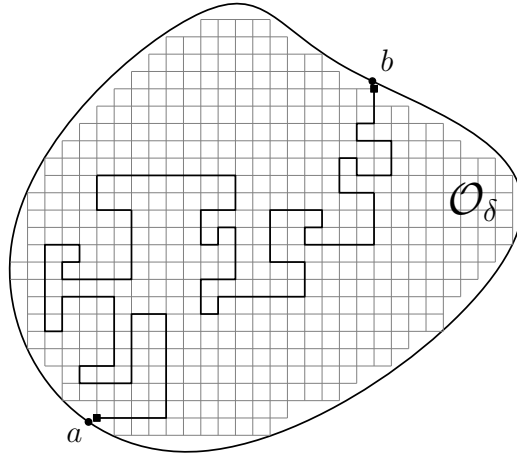
FIGURE 1. The path \gamma_\delta in (\mathcal{O}_\delta, a_\delta, b_\delta) .
