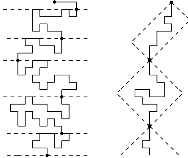
FIGURE 2. On the left, a bridge with its renewal points. On the right, a bridge with its diamond points (which we will shortly discuss).
