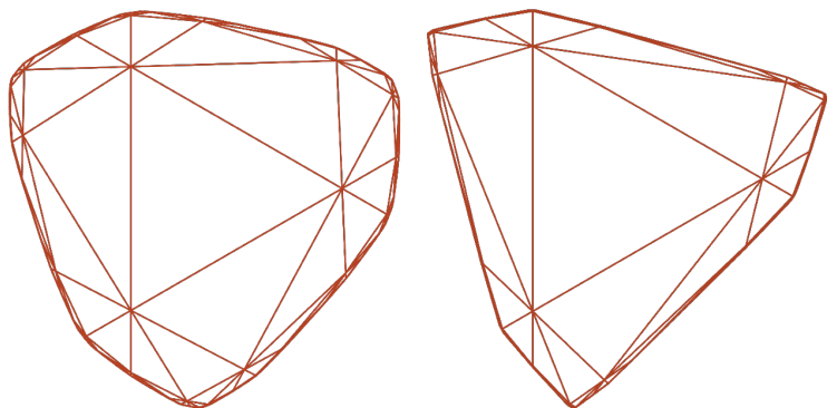
Two properly convex domains \Omega in the projective plane \mathbb{P}(\mathbb{R}^3) , with tilings by triangles. The symmetry groups of these tilings are discrete subgroups of G = \mathrm{SL}(3, \mathbb{R}) of infinite covolume, which are Anosov.
