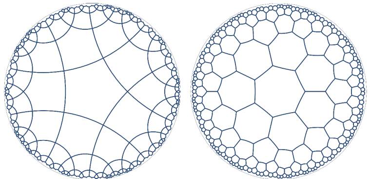
Tilings of the hyperbolic plane \mathbb{H}^2 : of valence 4 by regular pentagons (left), and of valence 3 by regular heptagons (right).
