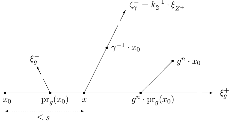
FIGURE 3. Illustration du lemme 3.3
